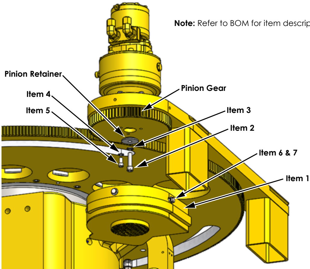
Figure 3: Guard Upgrade Kit Installation
