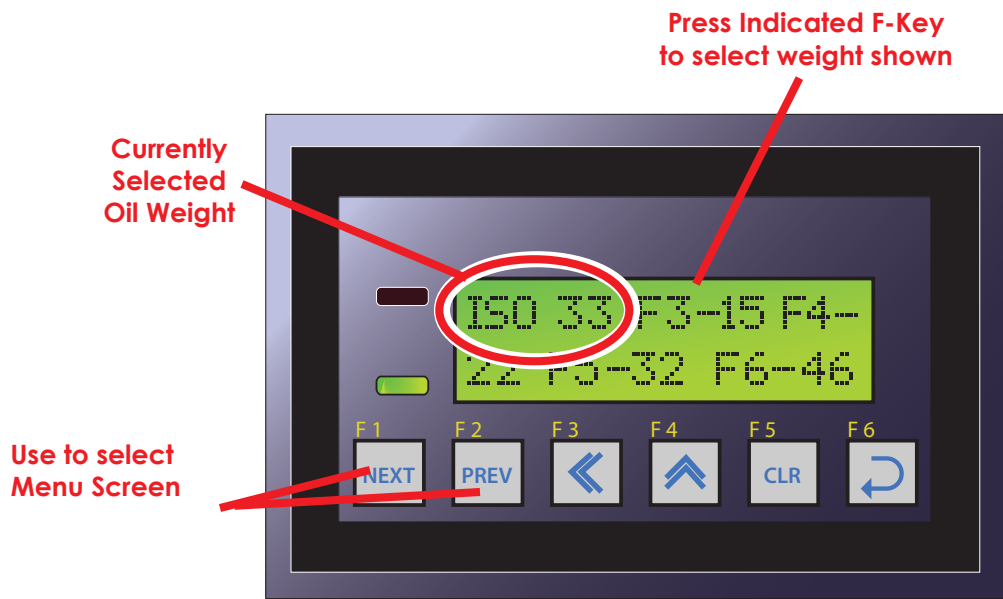
Figure 2: Catwalk Oil Selection Type Screen.
