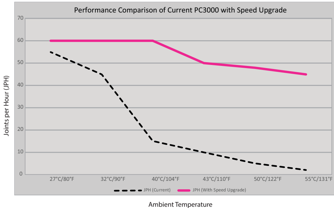
Figure 1: Current PC3000 Design Performance Compared with PC3000 Equipped with Speed Upgrade Kit AY52129 and latest PLC and HMI Upgrade
