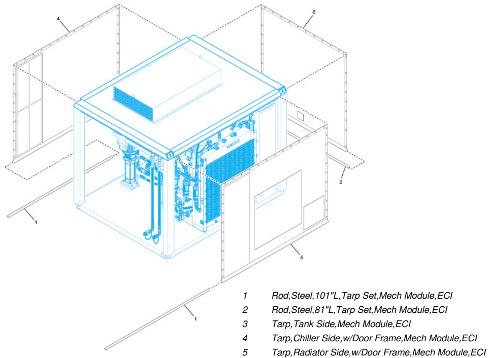
Figure 1 – Correct tarp set installation
